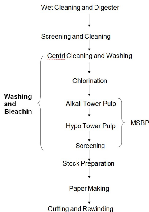
Fig. 3.1 PROCESS SEQUENCE FOR THE MANUFACTURE OF PAPER IN THE UNIT
