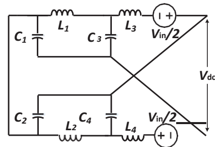
Fig. 7: Non-shoot-through state of the proposed Z-source inverter.
