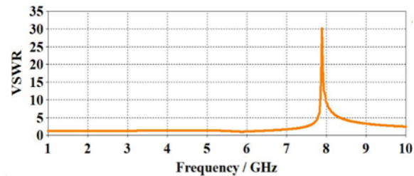
Fig.3 VSWR of the design
