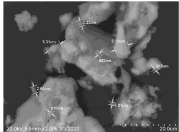
Figure 3:Nano Silica Powder+Cement
