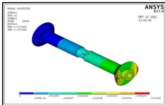
Fig 9: Resultant displacement of drive shaft.
