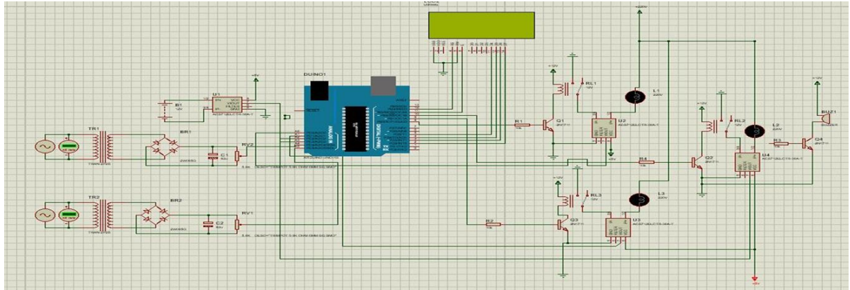
Fig 3. Circuit Diagram of Smart Control System for Senate Building, FUTO
