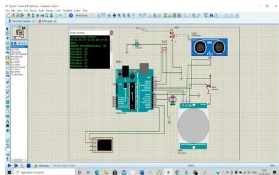
Fig. 7. Circuit Diagram with Simulation
