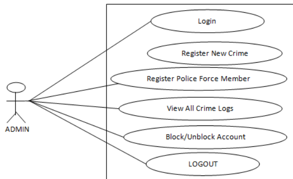
Figure 5: Use Case Diagram of Administrator Module
