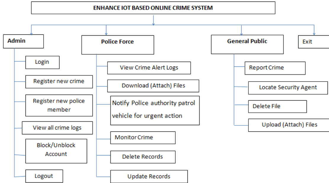
Figure 7: high level model of proposed system
