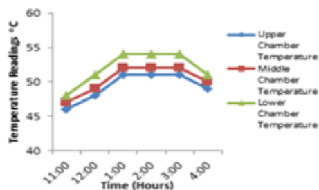
Fig 1. Maximum temperature profile of mirror at 45°C with drying chamber painted black
