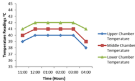
Fig 4. Maximum Temperature Profile at No Mirror
