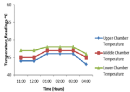
Fig 2. Maximum Temperature Profile Of Mirror at 45°C
