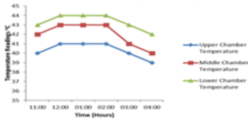
Fig 3. Maximum Temperature profile of Mirror at 25°C
