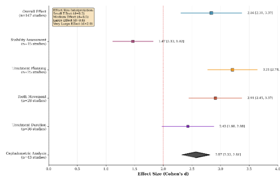
Figure 2. Forest Plot: Effect Sizes for AI vs Traditional Methods Orthodontic Treatment Outcome Prediction
