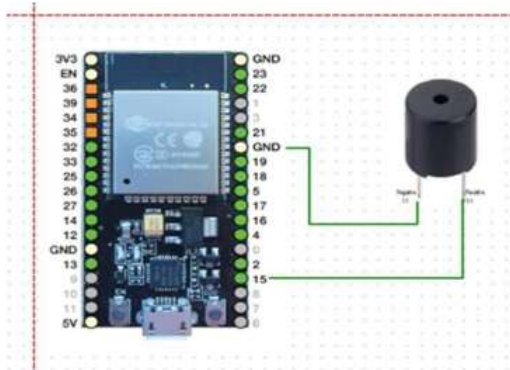
Fig 4: Controller side Connection Software Flow
