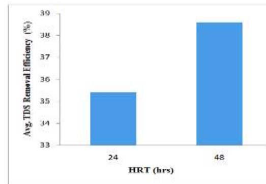
Figure 3.4: TDS removal efficiency
