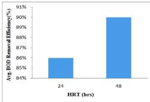
Figure 3.1: BOD removal efficiency
