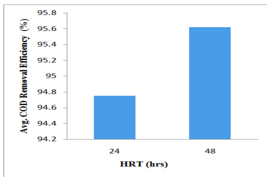
Figure 3.2: COD removal efficiency
