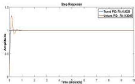
Fig. 2: Unit step response using: tuned PID and untuned PID
