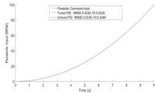
Fig. 4: Parabolic input command
