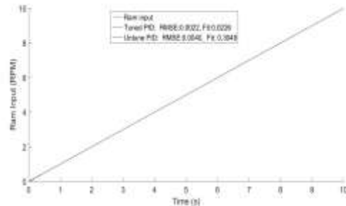
Fig. 5: Ram input command
