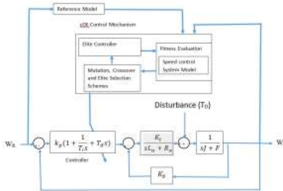
Fig. 1: Block diagram of the speed control system
