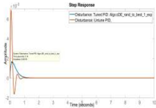
Fig. 6: Disturbance step response
