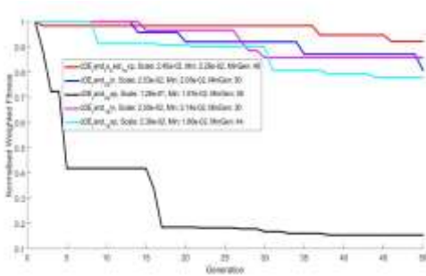
Fig. 7: Generational fitness function of the cDE variants used
