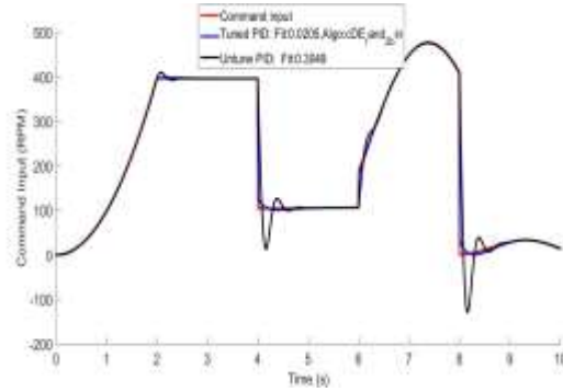
Fig. 3: Real world command input using tuned and untuned PID
