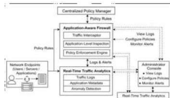
Figure 1. Architecture Diagram
