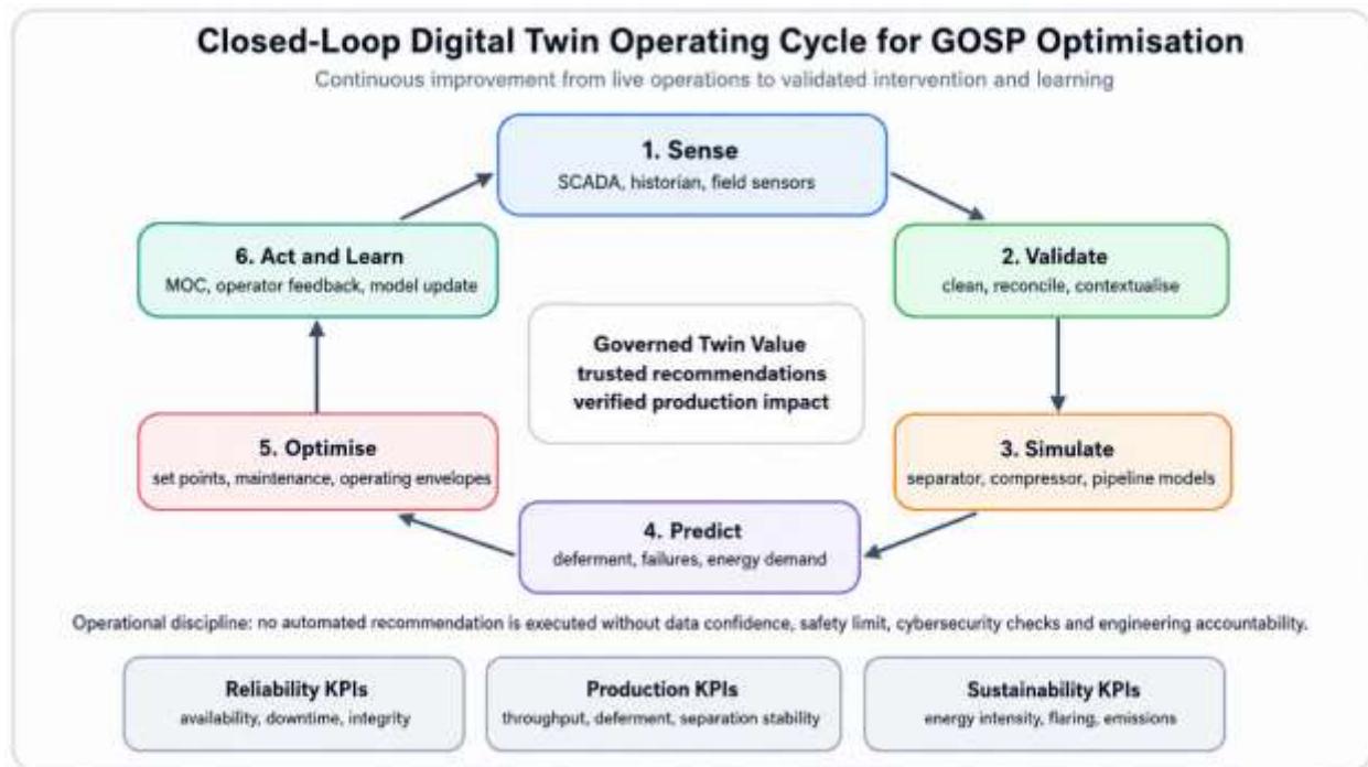
Figure 2. Development, validation and controlled deployment workflow for a GOSP digital twin.
