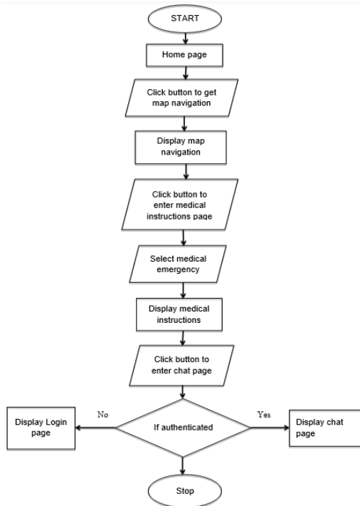
Fig. 3. The Flow Chart Illustrating the Emken System
